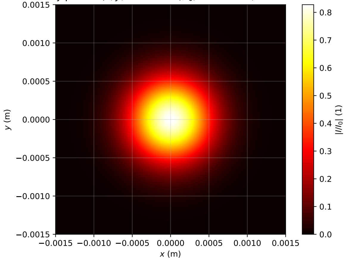
Intensity profile I(x, y, z = 1.035m)/I_0 , Pin=0.1Pcr, artificial time
